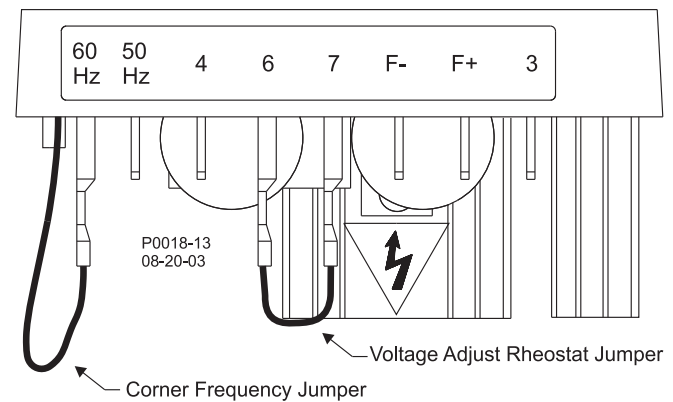
Figure 3 - Jumper Locations
