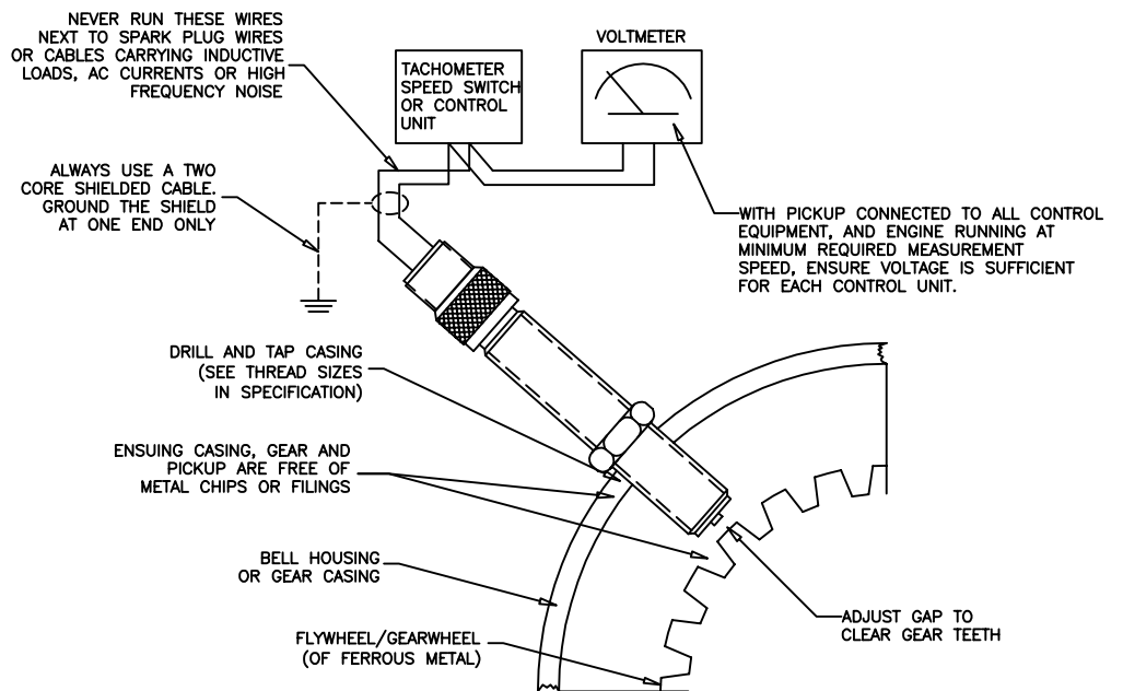
TYPICAL INSTALLATION
