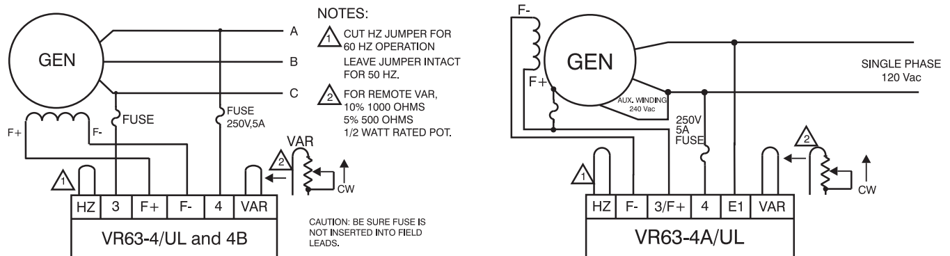
Figure 2 - Typical Interconnection Diagram
