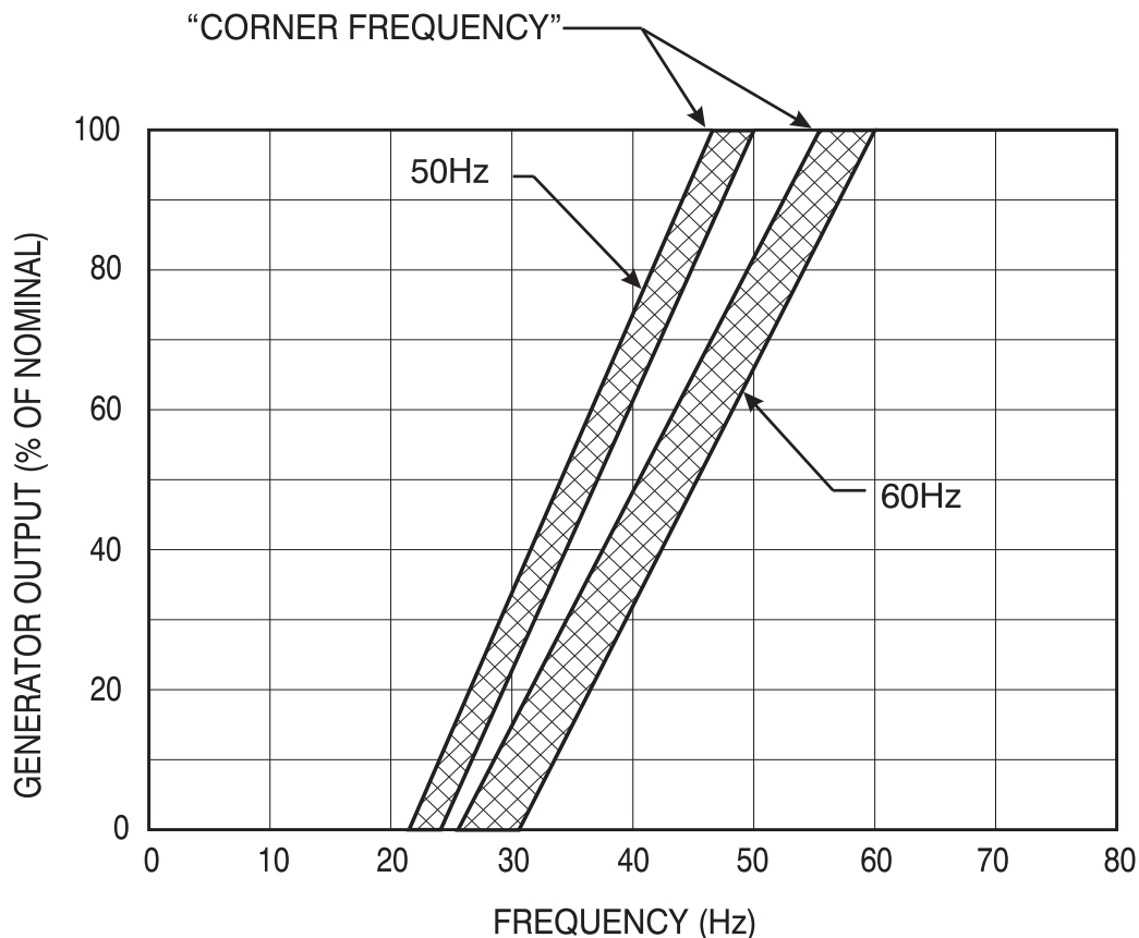
Figure 1 - Frequency Compensation Characteristic
