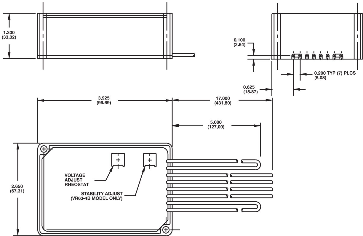
Figure 3 - Outline Drawing
